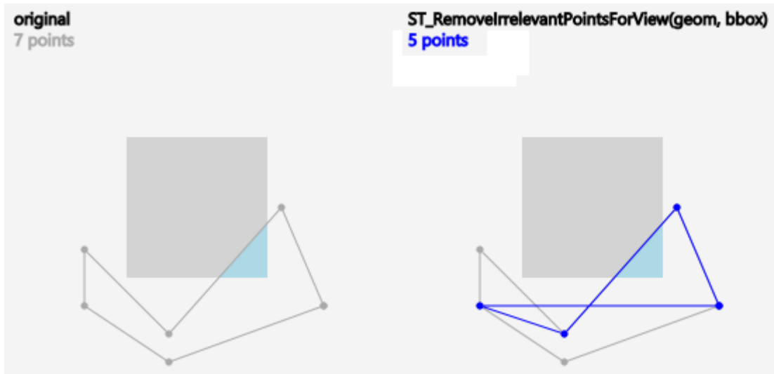
Example: Due to the fact that points are just sorted out and no new points are computed, the result of ST_RemoveIrrelevantPointsForView() may contain self-intersections.
