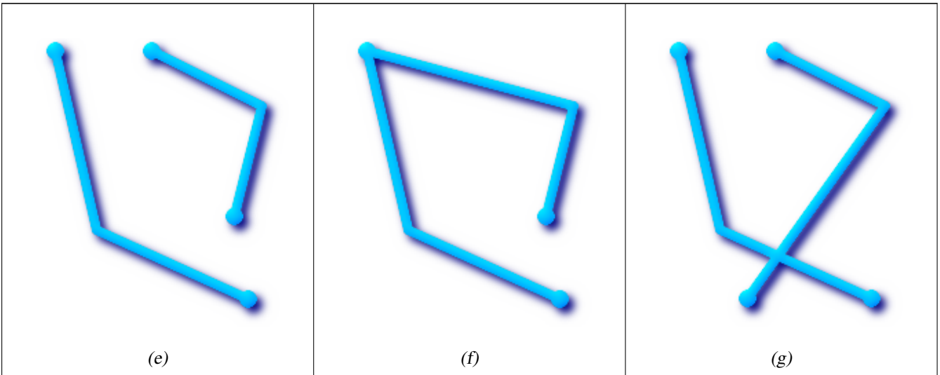
(e) and (f) are simple MULTILINESTRINGs, (g) is not.
